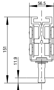
2車カーテンランナー=LW / 2-Wheel Curtain Runner = LW
